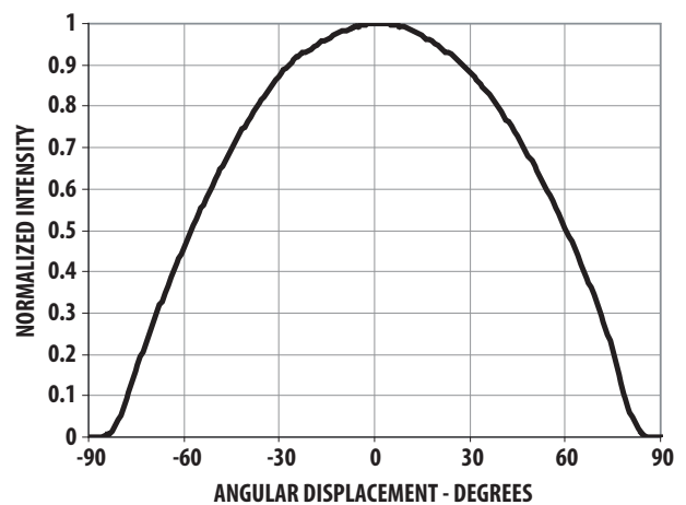
Figure 8. Radiation Pattern
